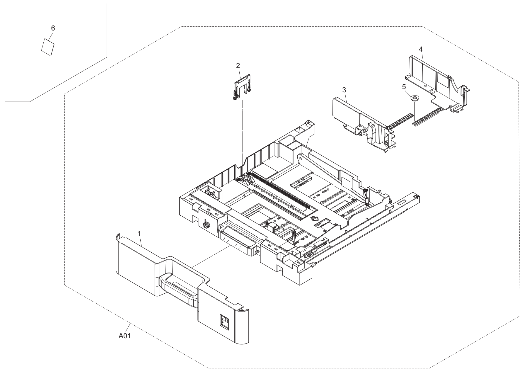
FIG. 4 Paper Cassette
