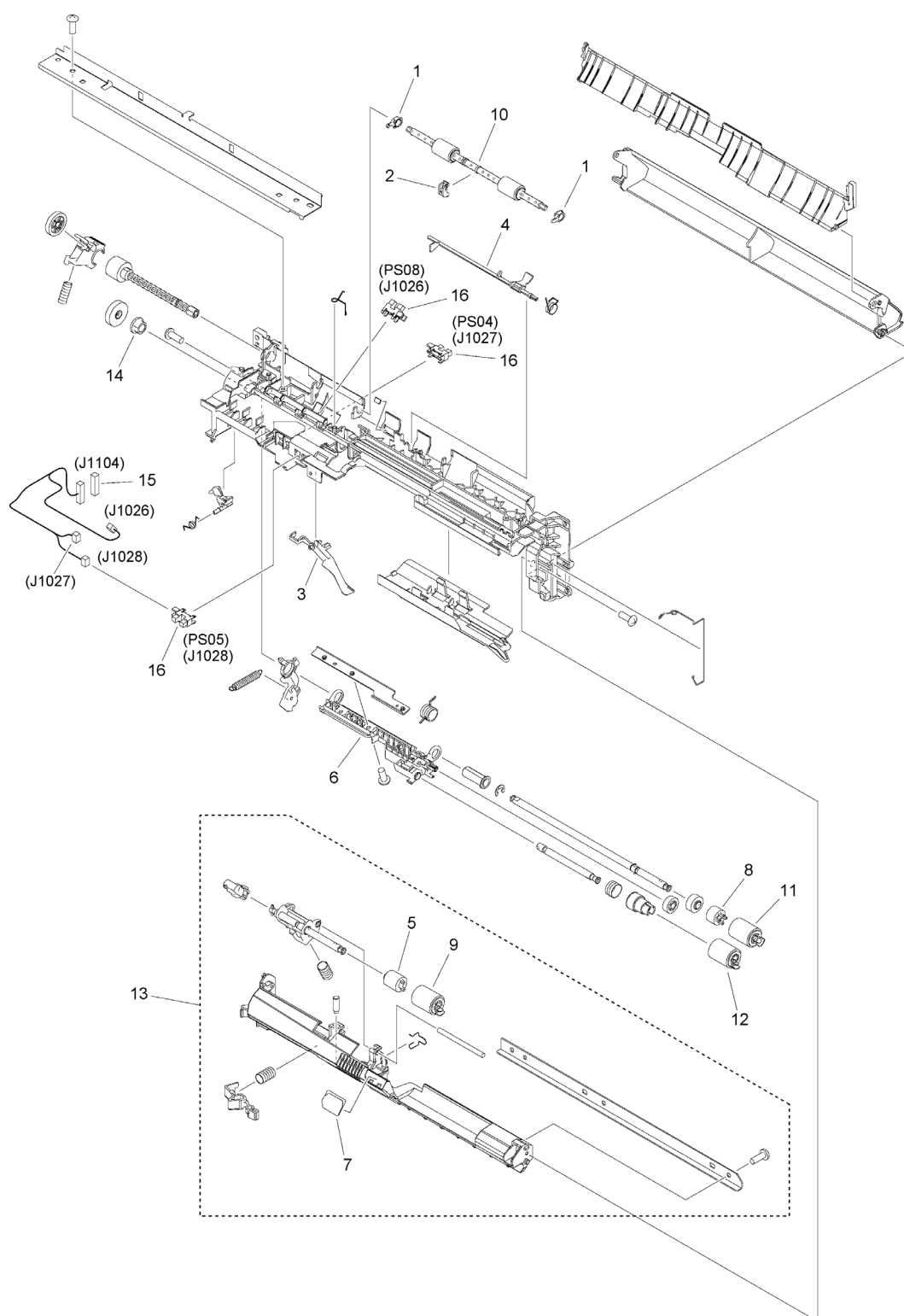
Figure 310 PAPER PICK-UP ASSEMBLY (SMALL)
