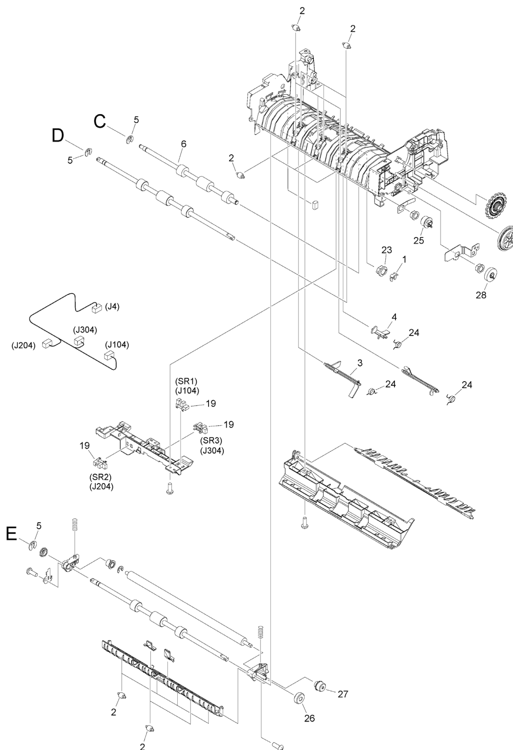
Figure C41 (2/2) PAPER FEED ASSEMBLY (DADF-BA1 model )
