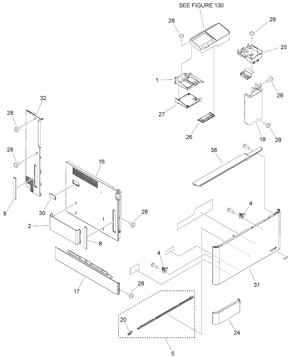
Figure 100E (1/2)EXTERNAL COVERS, PANELS, ETC.
