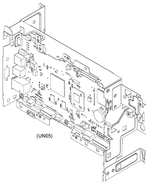
Figure 930A MAIN CONTROLLER PCB ASSEMBLY (C3125 Series)
