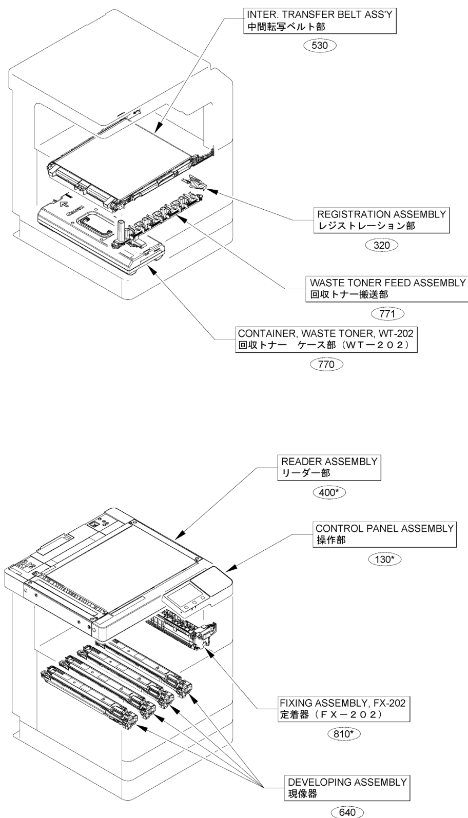
Figure A1A (3/5) ASSEMBLY LOCATION DIAGRAM
