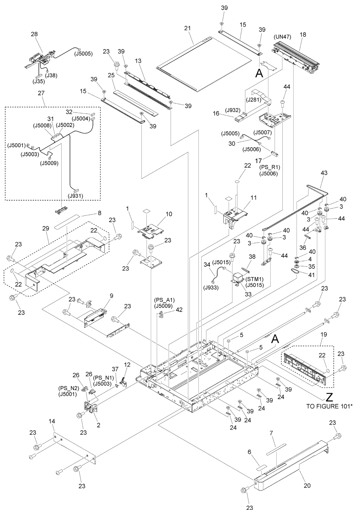
Figure 400B READER ASSEMBLY
