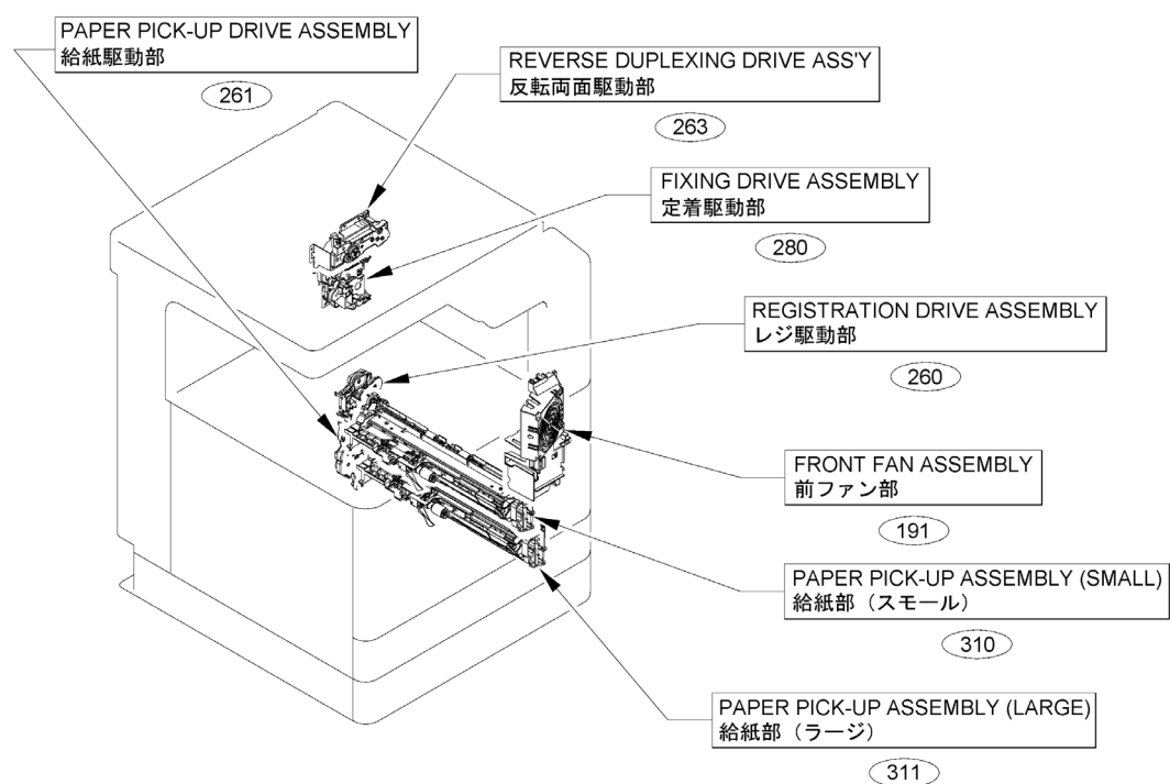
Figure A1A (2/5) ASSEMBLY LOCATION DIAGRAM
