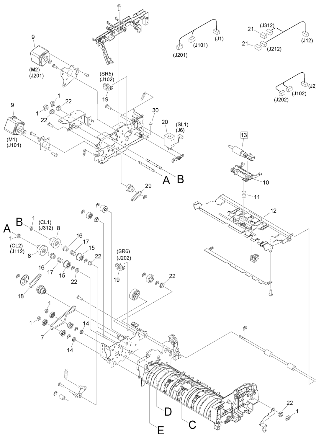
Figure C41 (1/2) PAPER FEED ASSEMBLY (DADF-BA1 model )
