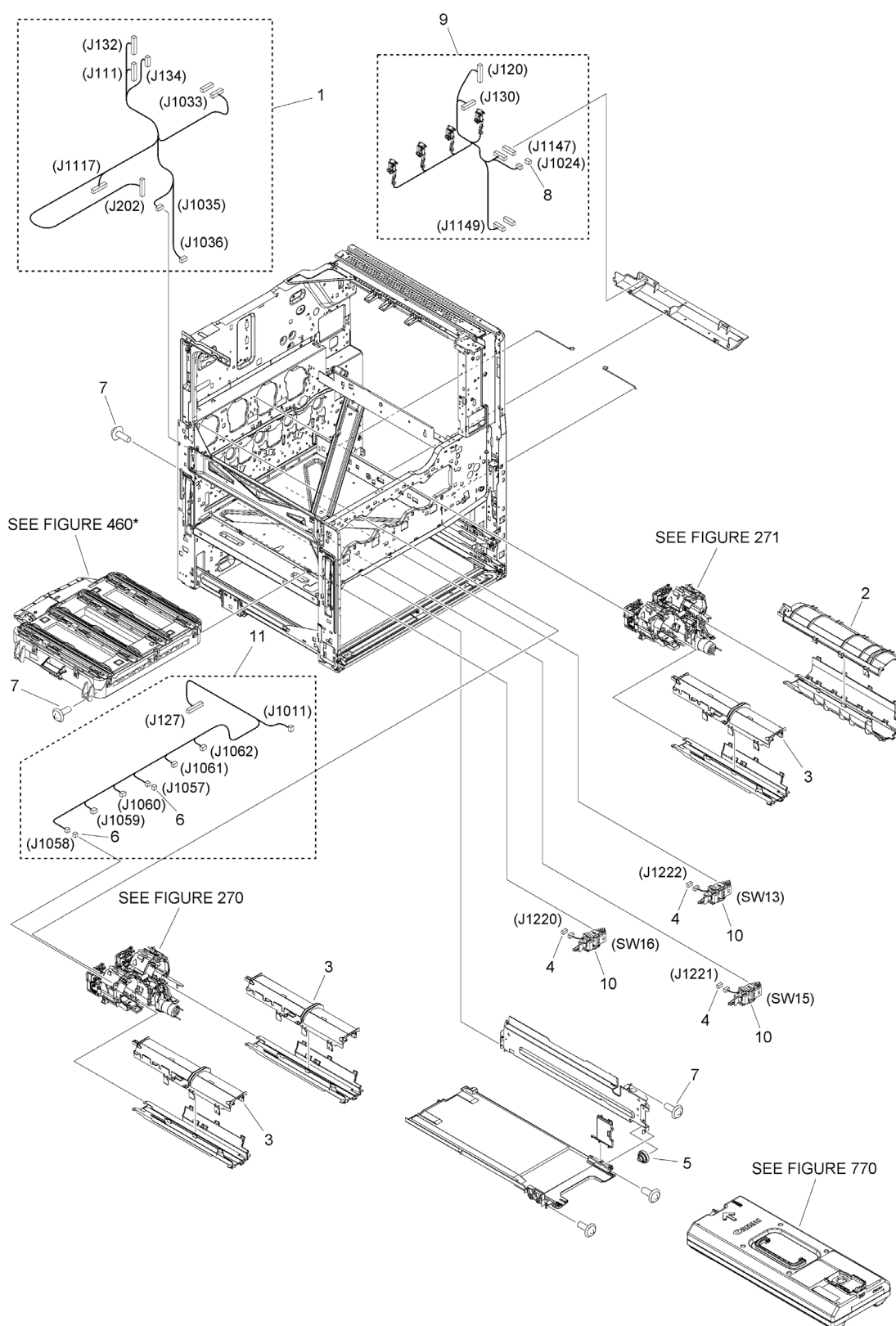
Figure 103 EXTERNAL COVERS, PANELS, ETC.
