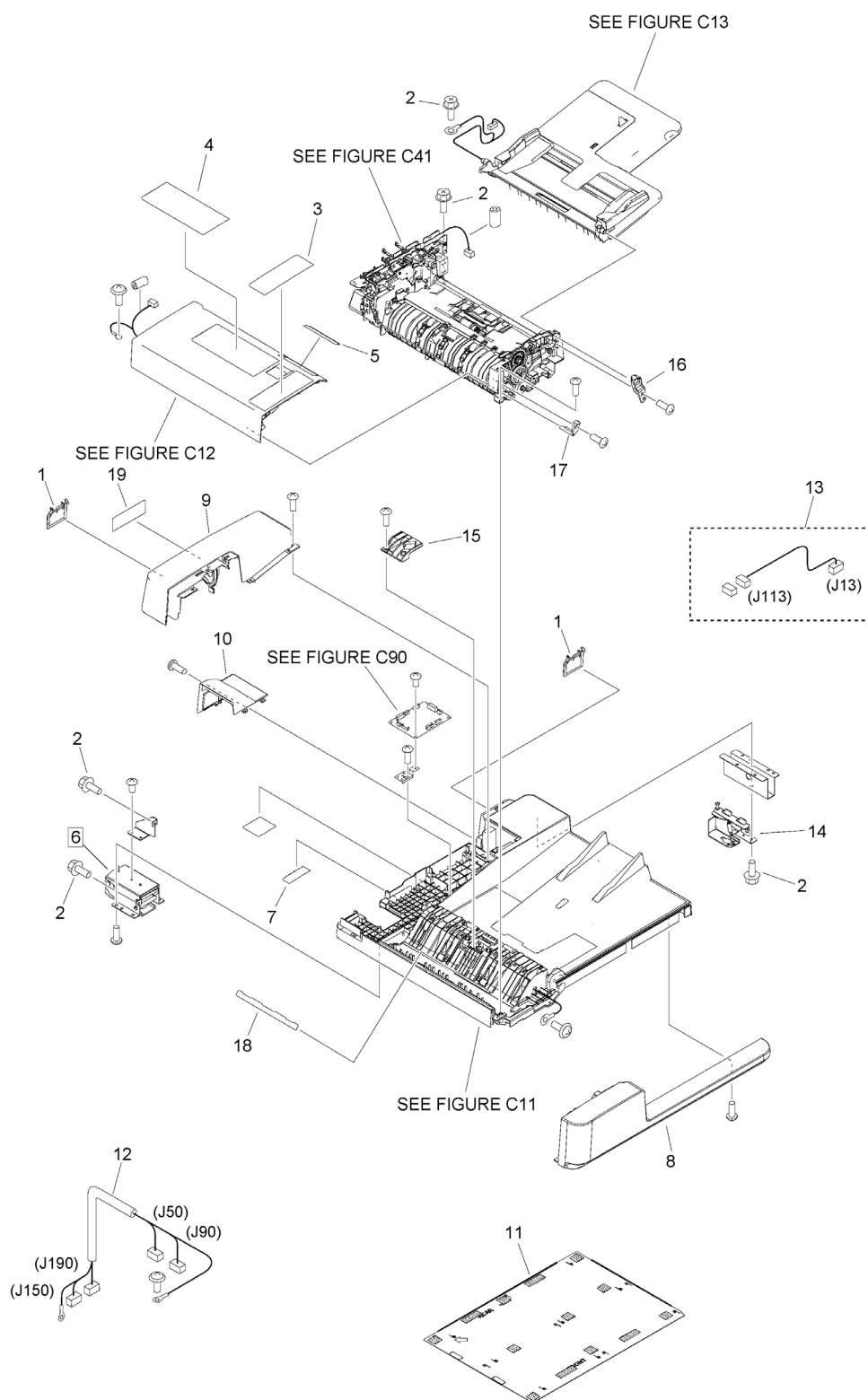
Figure C10 INTERNAL COMPONENTS (DADF-BA1 model)
