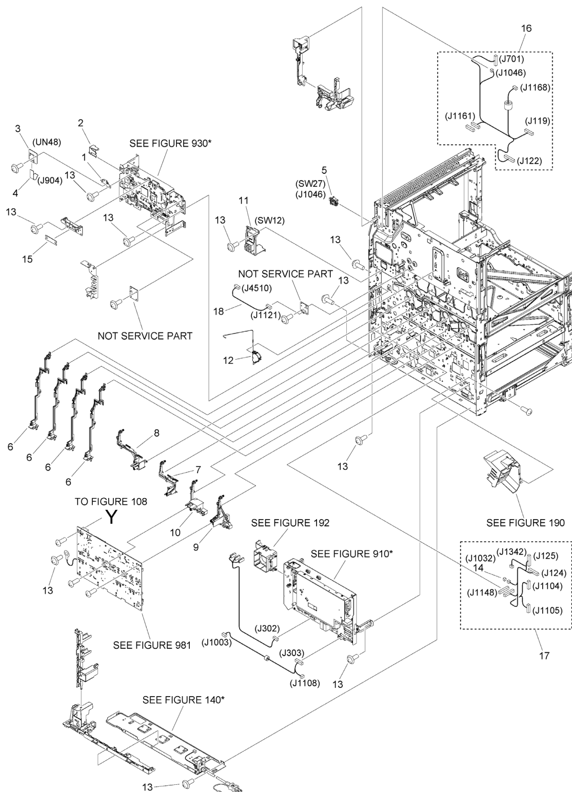
Figure 107A MACHINE REAR PLATE 1
