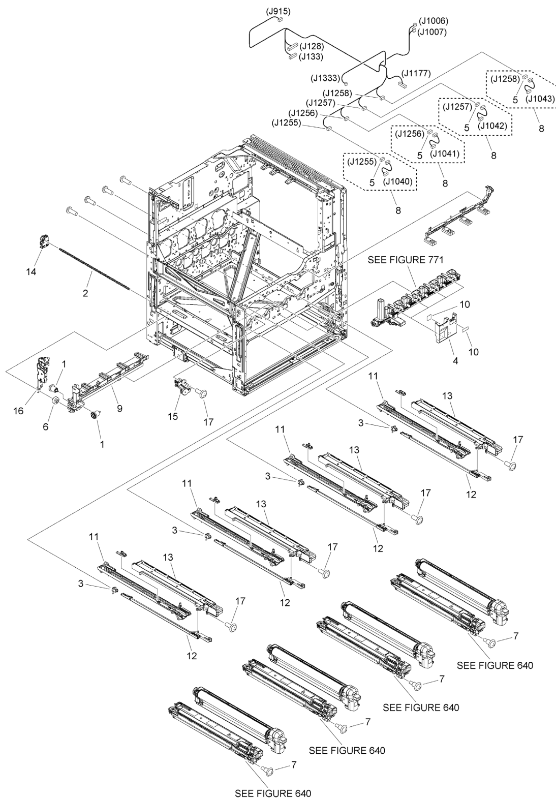
Figure 102B INTERNAL COMPONENTS 2
